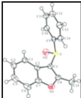
Fig. 1. The molecular structure of the title compound, showing displacement ellipsoids drawn at the 50% probability level.
